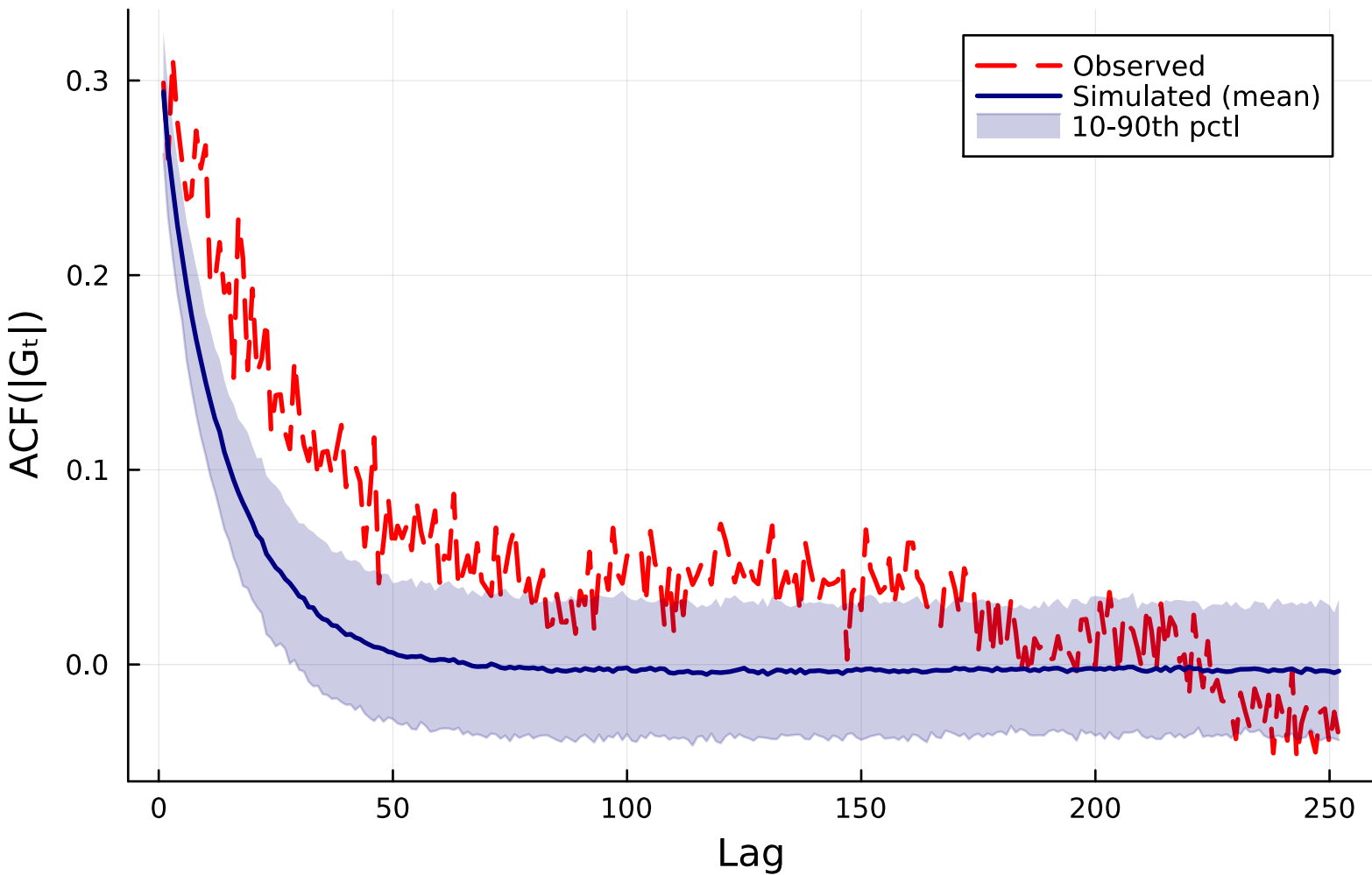
ACF( |G_t| ) at Optimal — K=11 ( \epsilon=0.0001 , \lambda=10 )
