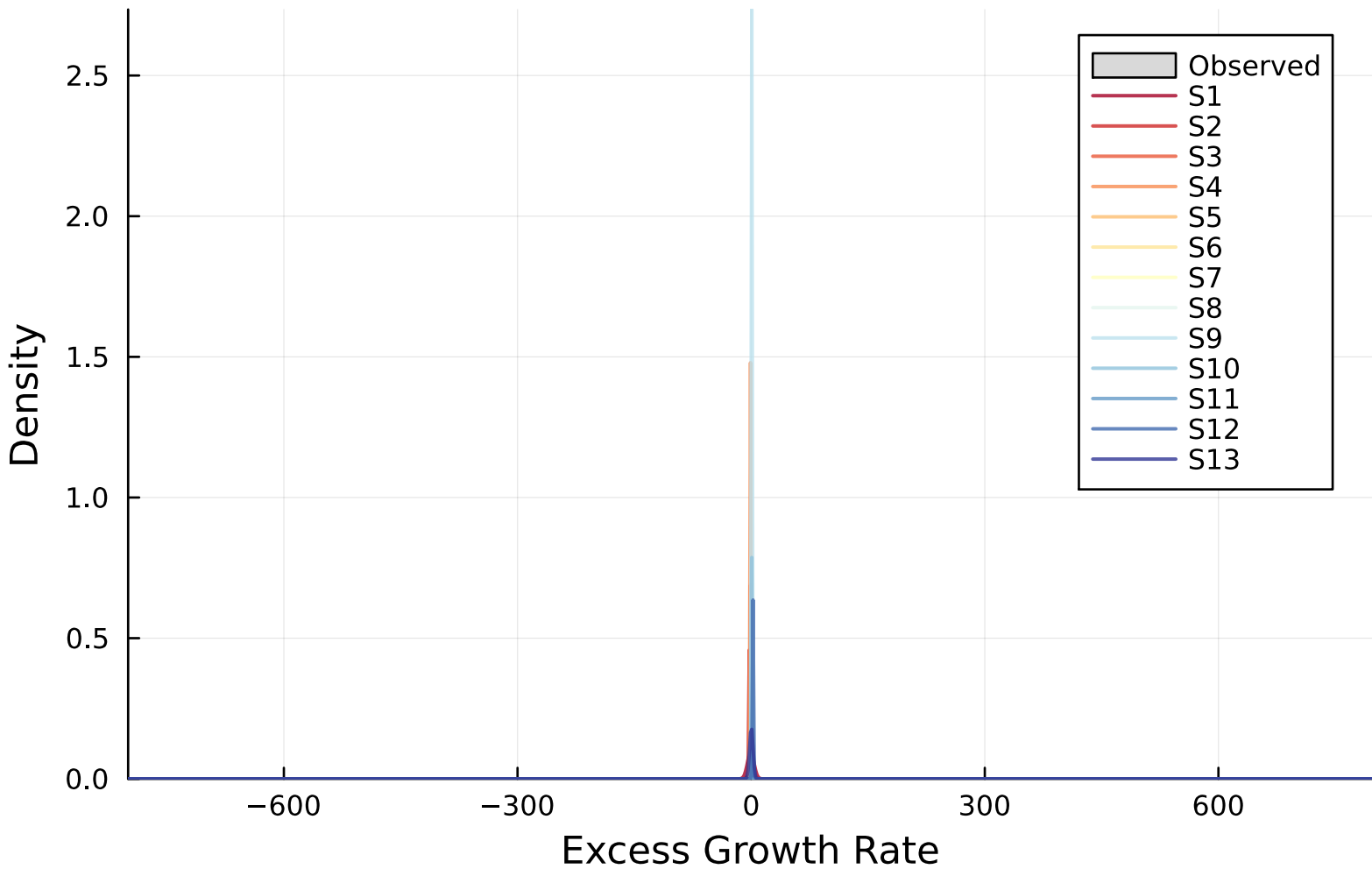
Emission Distributions (SPY, K=13)
