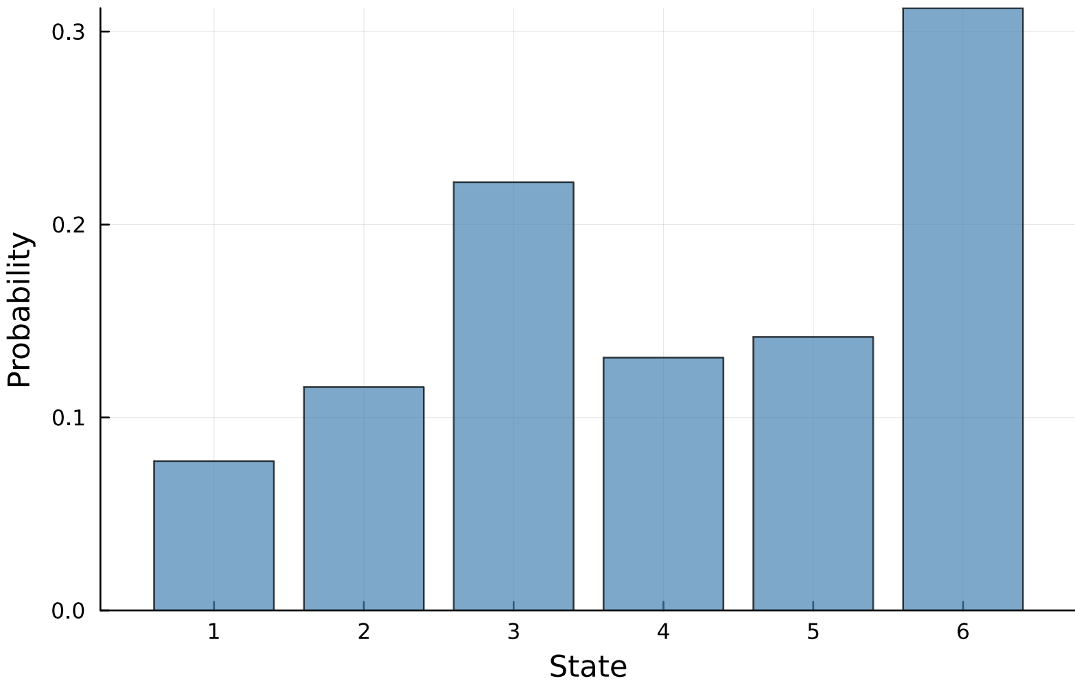
Stationary Distribution \pi — K=6
