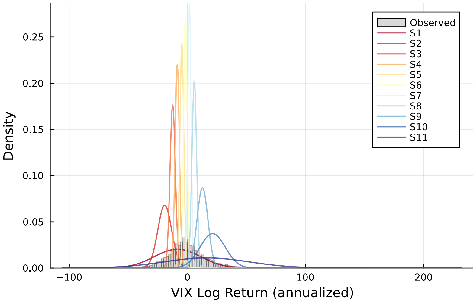
Emission Distributions (VIX, K=11)
