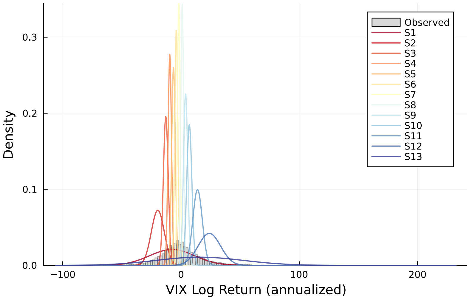
Emission Distributions (VIX, K=13)
