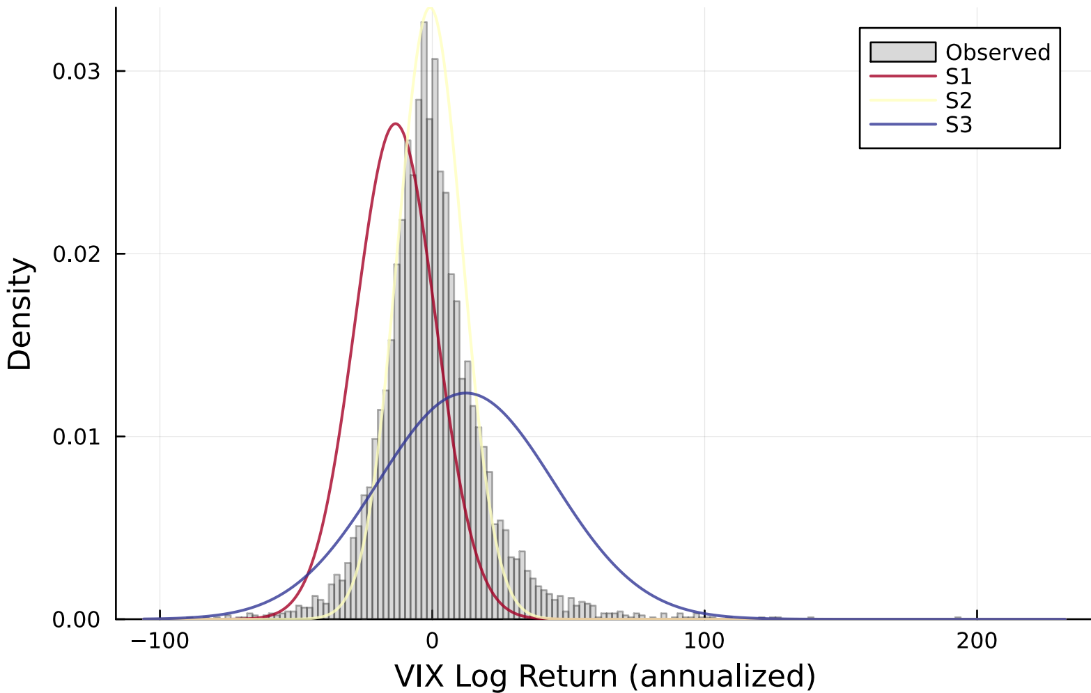
Emission Distributions (VIX, K=3)
