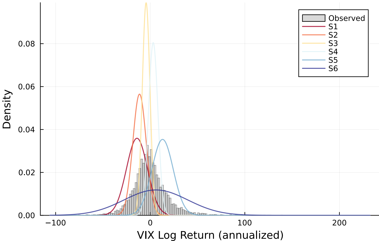
Emission Distributions (VIX, K=6)
