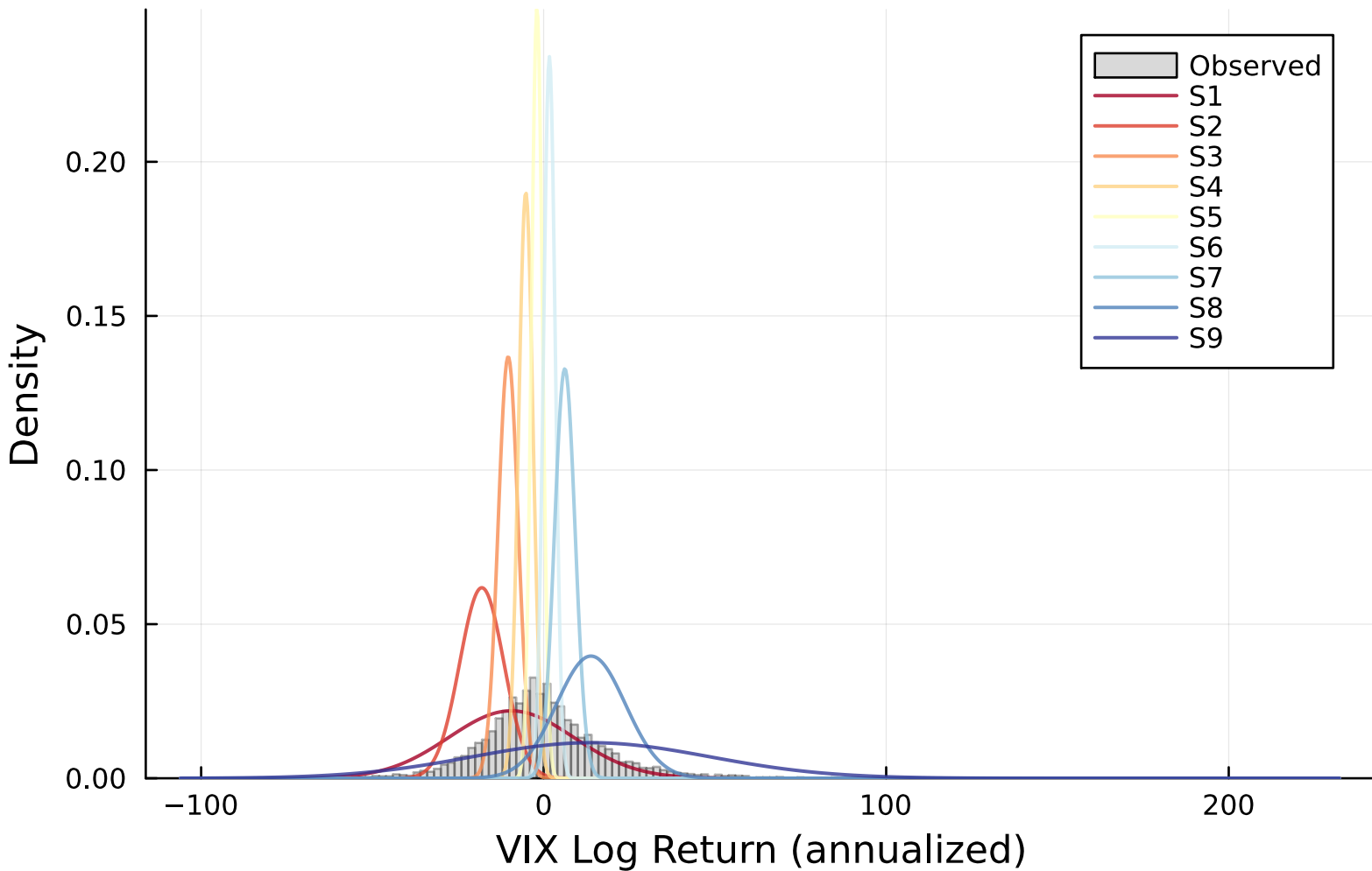
Emission Distributions (VIX, K=9)
