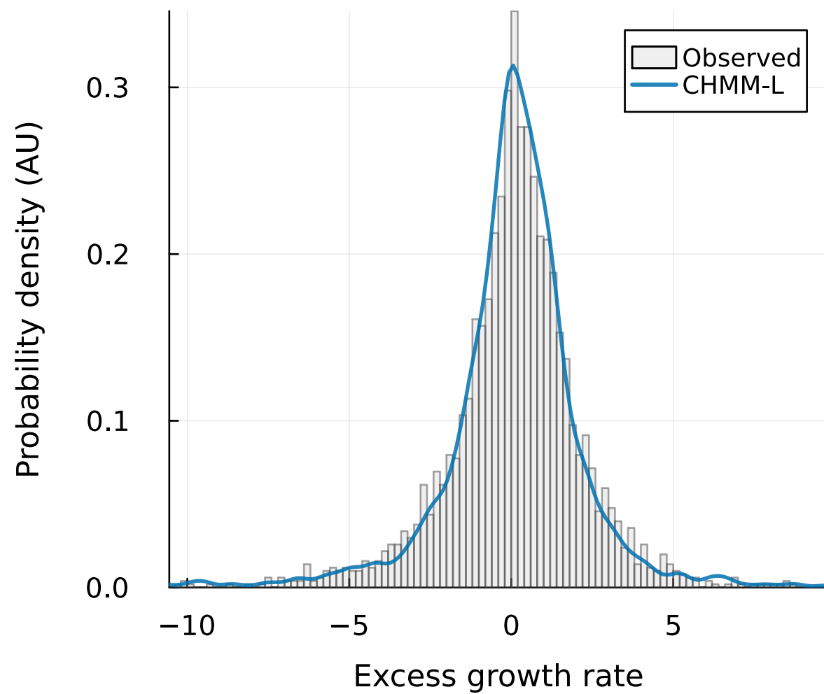
(a) IS density (KS: 95.3%)
