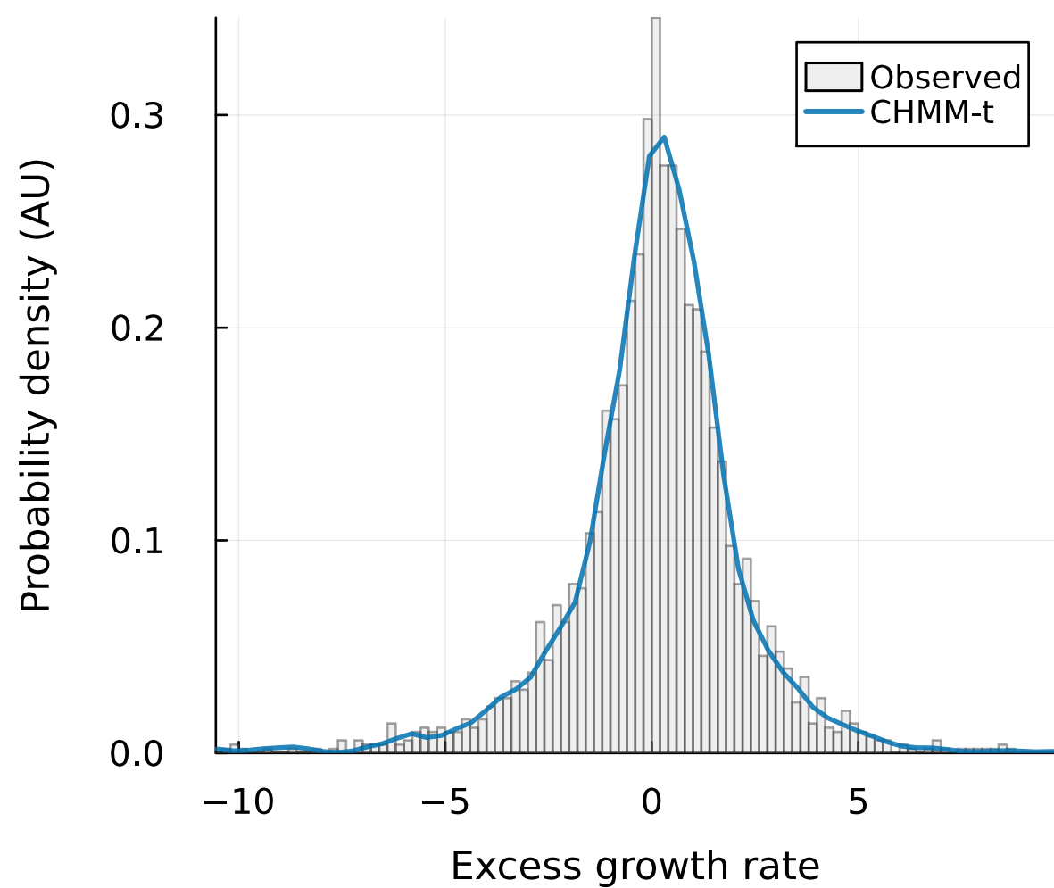
(a) IS density (KS: 95.7%)
