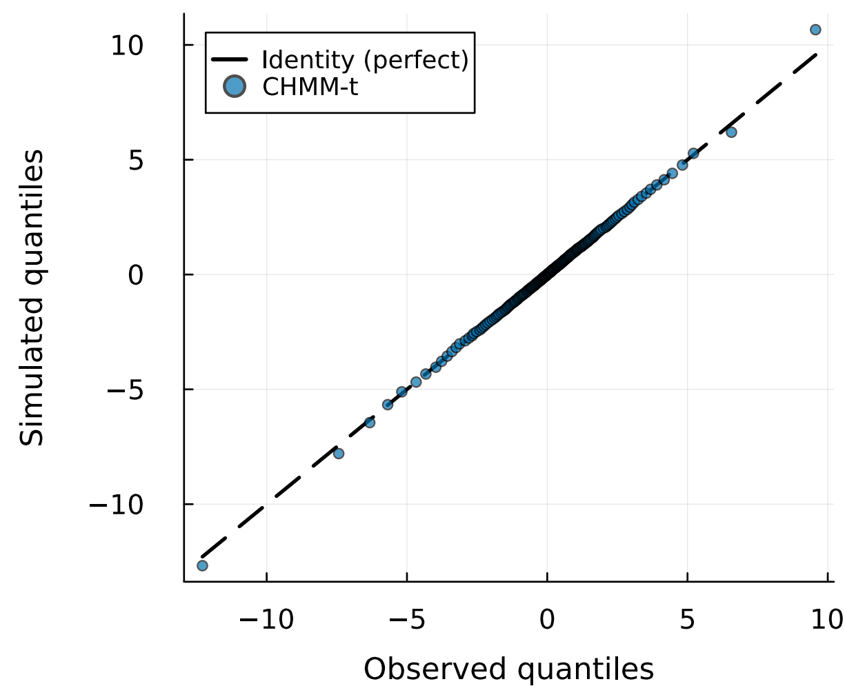
(c) Tail Q-Q plot (0.1st-99.9th)
