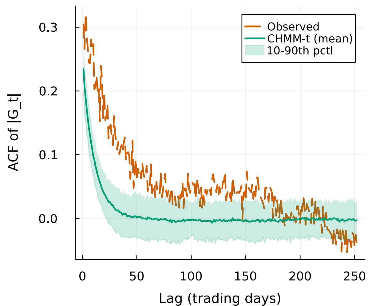
(b) ACF of |G_t|
