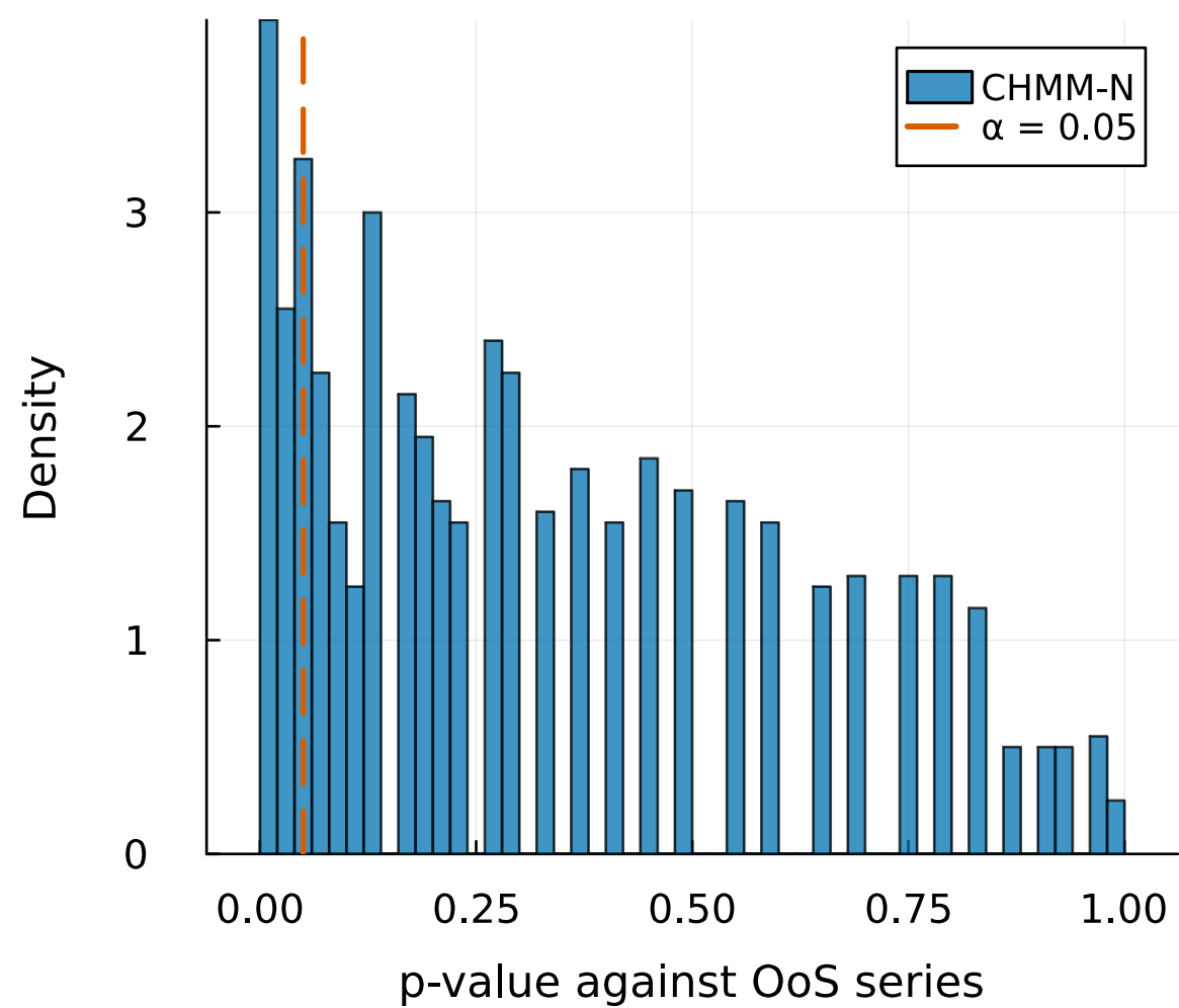
(a) OoS KS p-values (pass: 83.2%)
