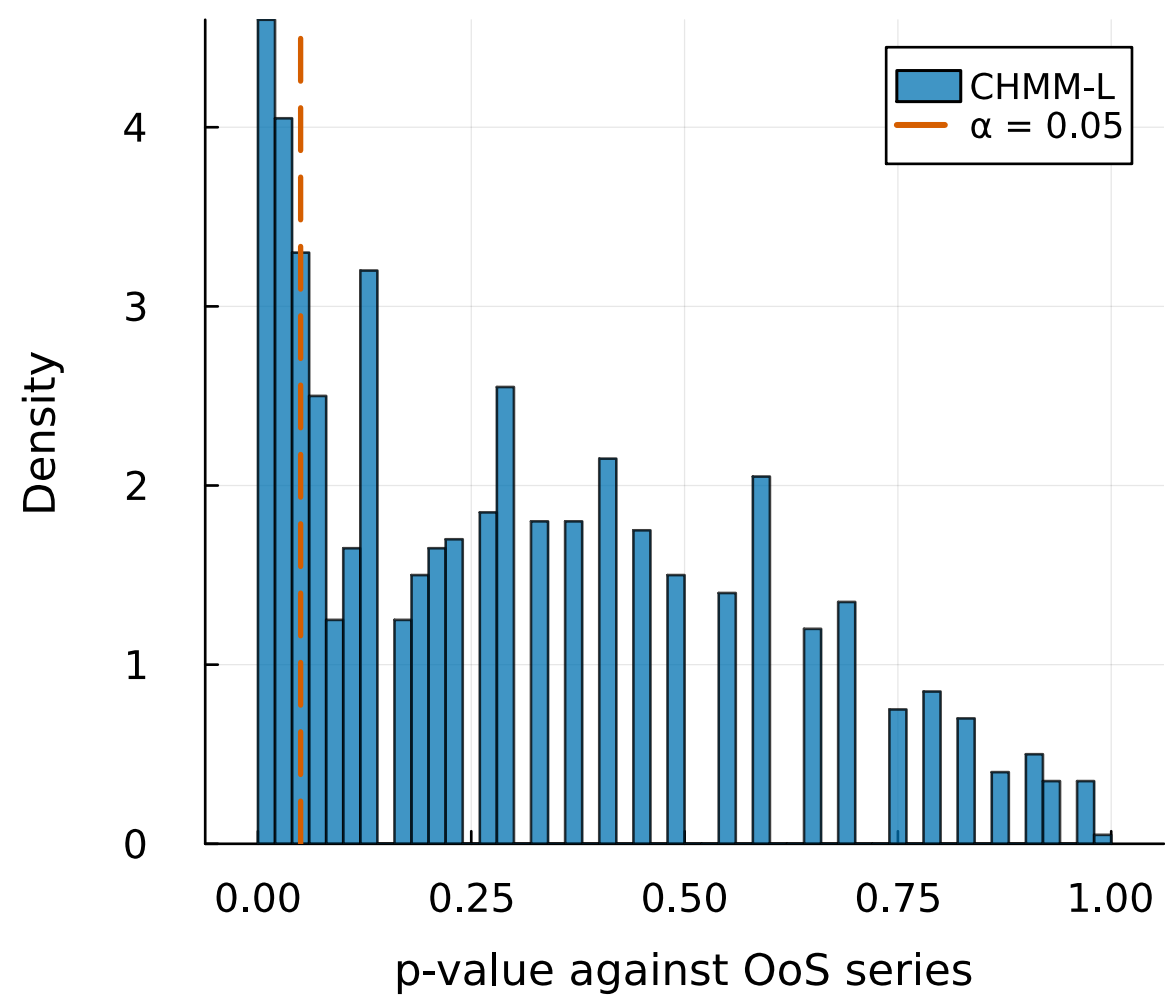
(a) OoS KS p-values (pass: 77.9%)
