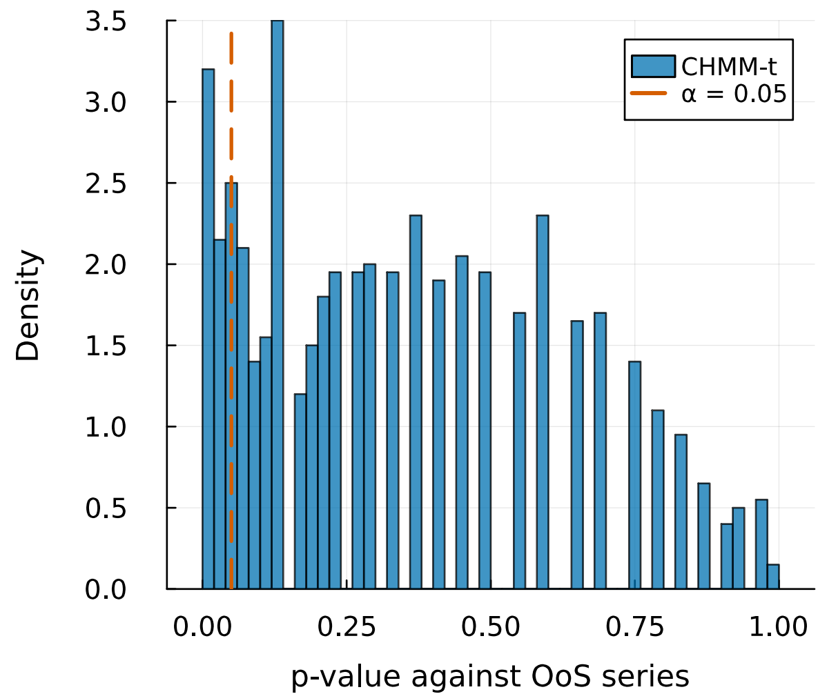
(a) OoS KS p-values (pass: 86.2%)
