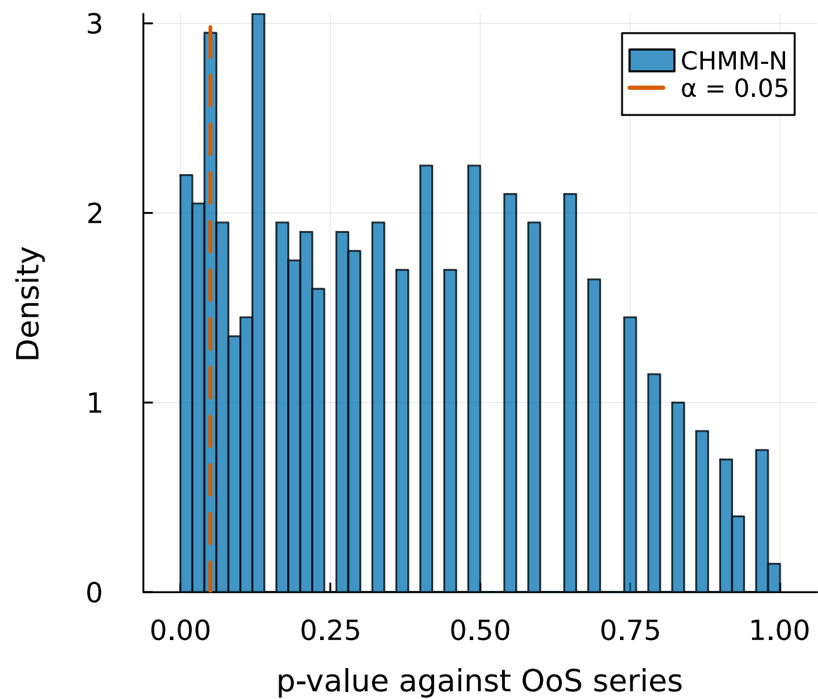
(a) OoS KS p-values (pass: 87.3%)
