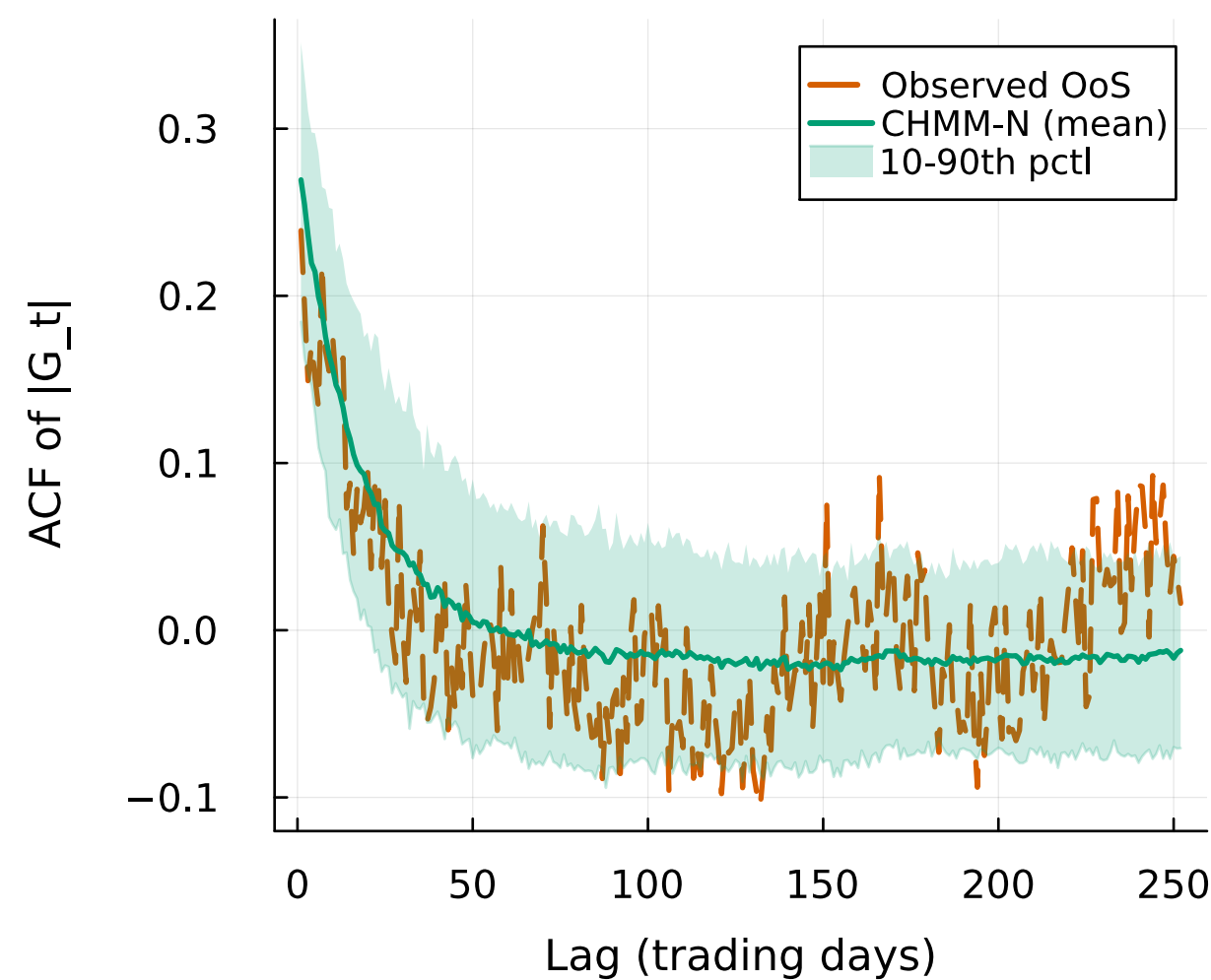
(c) OoS ACF of |G_t|
