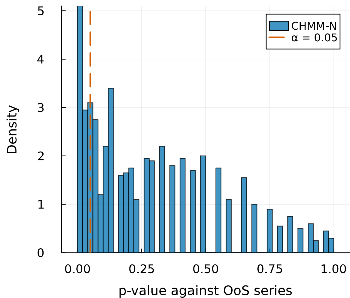
(a) OoS KS p-values (pass: 79.7%)
