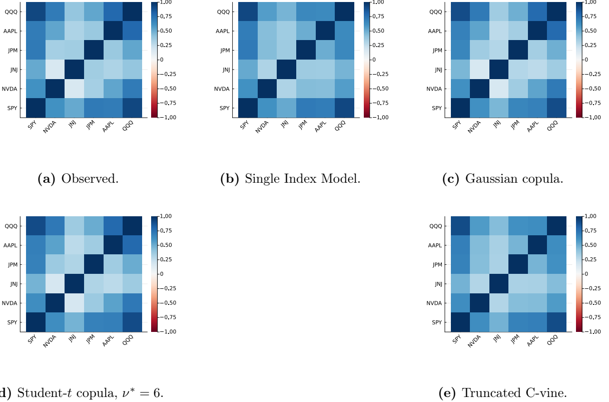
Figure 30. Cross-asset IS correlation reproduction across dependence models (Pipeline B, companion to Table 67). Panel (a): observed correlation matrix on 2014-01-03 through 2024-01-03 daily excess log returns for SPY, NVDA, JNJ, JPM, AAPL, QQQ (IS window, T_{IS} = 2,516 ). Panel (b): path-averaged correlation under the Single Index Model with SPY as market factor. Panel (c): path-averaged correlation under the Gaussian copula on CHMM marginals. Panel (d): path-averaged correlation under the Student- t copula on CHMM marginals, \nu^* = 6 . Panel (e): path-averaged correlation under a truncated C-vine copula with SPY as root. Each simulated panel averages over 200 paths of length T_{IS} . All marginals are the per-asset CHMM-N fits at K = 18 from Table 7; color scale in [-1, 1] , red-white-blue (RdBu) diverging. Closer visual match to panel (a) is better.
