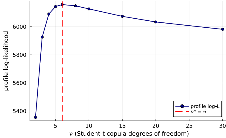
Figure 29. Profile log-likelihood of the Student-t copula used inside Pipeline B on the six-asset SPY cross-section (SPY, NVDA, JNJ, JPM, AAPL, QQQ; IS window 2014-01-03 through 2024-01-03). The vertical axis is the profile log-likelihood evaluated at each degrees-of-freedom value \nu on the grid \{2, 3, 4, 5, 6, 8, 10, 15, 20, 30\} ; the dashed red line marks the profile MLE \nu^* = 6 (peak value 6157.47). The CHMM-N marginals are held fixed at the Pipeline A per-asset fits while \nu is varied.
