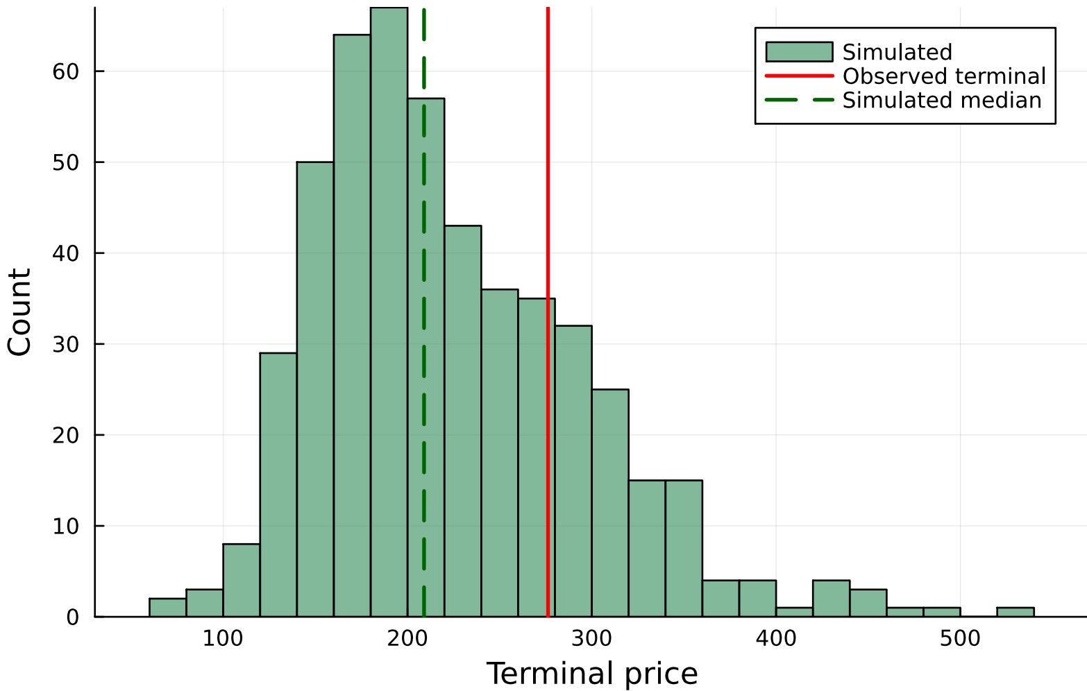
AAPL - VIX-cond. CHMM-N terminal (n=500)
