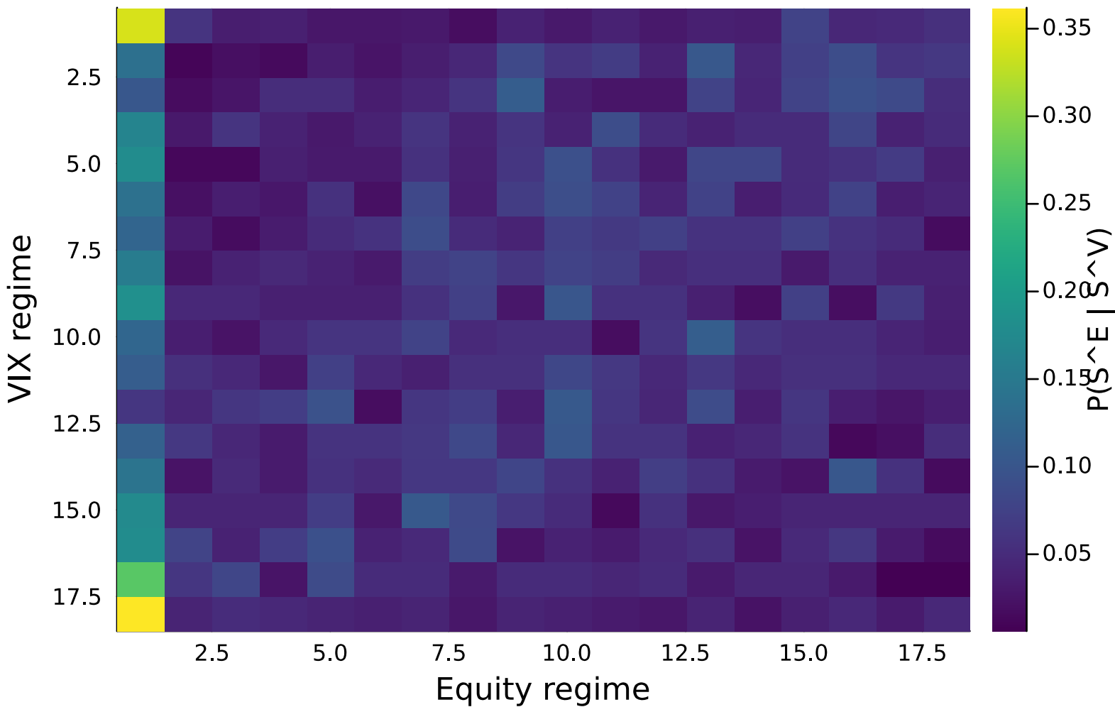
AAPL coupling C[s^{\sim}V, s^{\sim}E] (lag h=1 , Laplace \alpha=1.0 )
