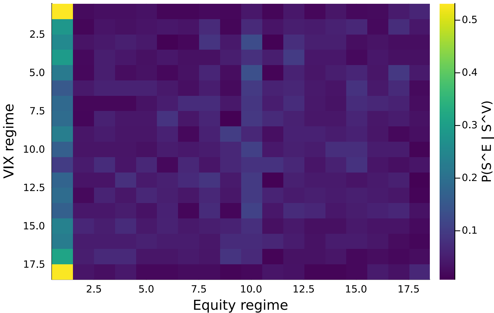
JPM coupling C[s^V, s^E] (lag h=1 , Laplace \alpha=1.0 )
