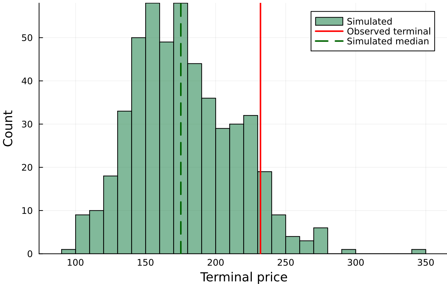
JNJ - VIX-cond. CHMM-N terminal (n=500)
