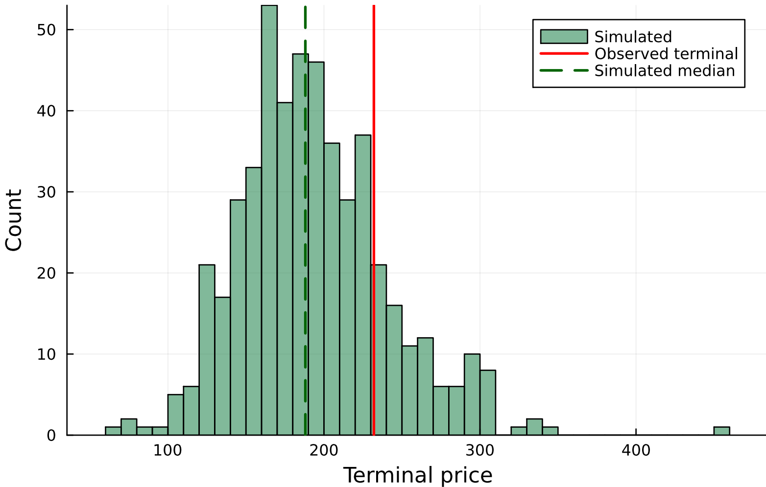
JNJ - VIX-cond. CHMM-t terminal (n=500)
