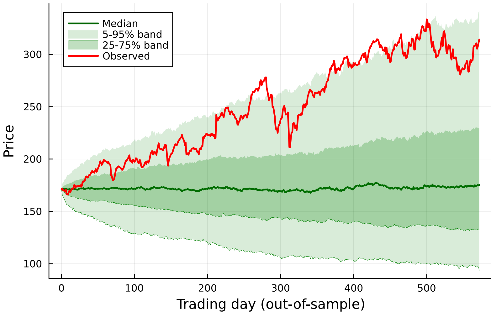
JPM - VIX-cond. CHMM-t (K=18, 500 paths, lag=1)
