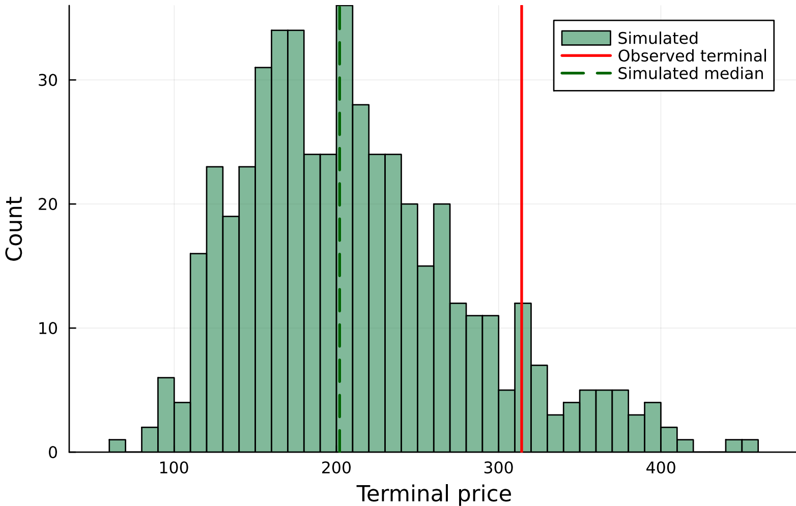
JPM - VIX-cond. CHMM-N terminal (n=500)
