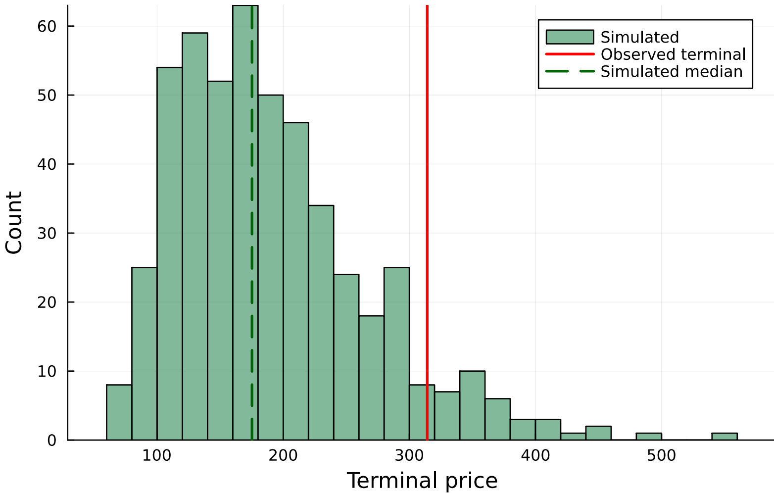
JPM - VIX-cond. CHMM-t terminal (n=500)
