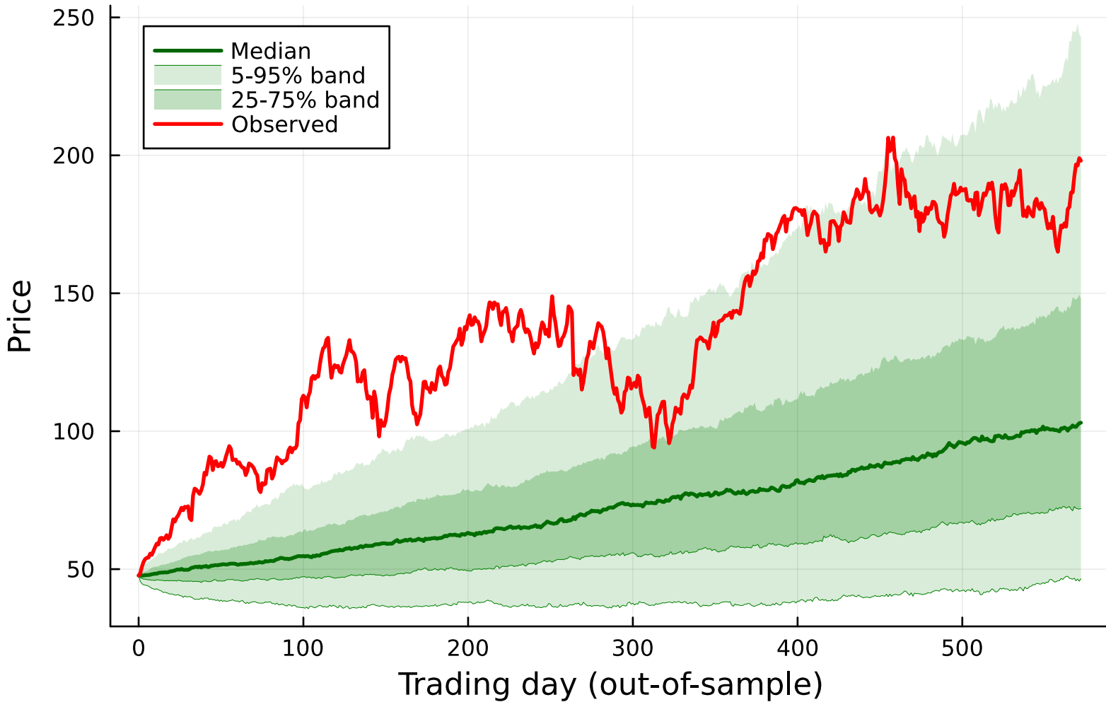
NVDA - VIX-cond. CHMM-N ( K=18 , 500 paths, lag=1)
