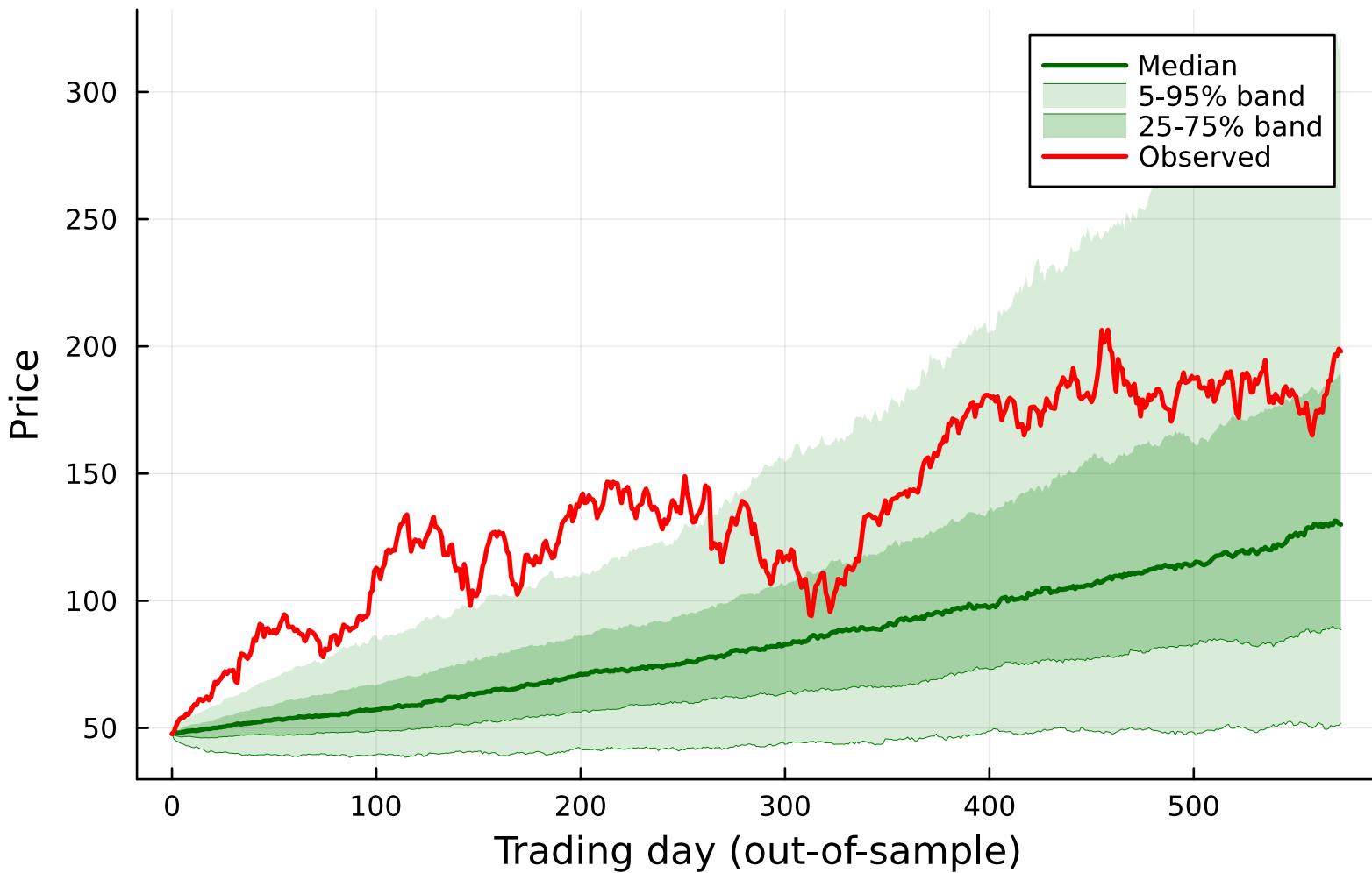
NVDA - VIX-cond. CHMM-t (K=18, 500 paths, lag=1)
