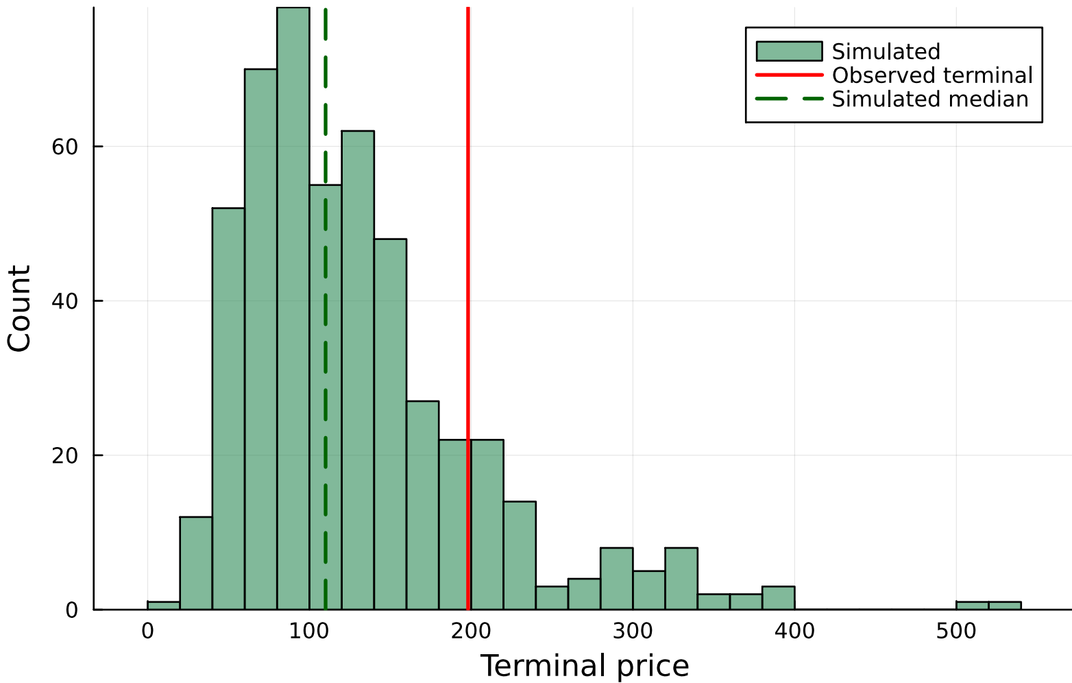
NVDA - VIX-cond. CHMM-L terminal (n=500)
