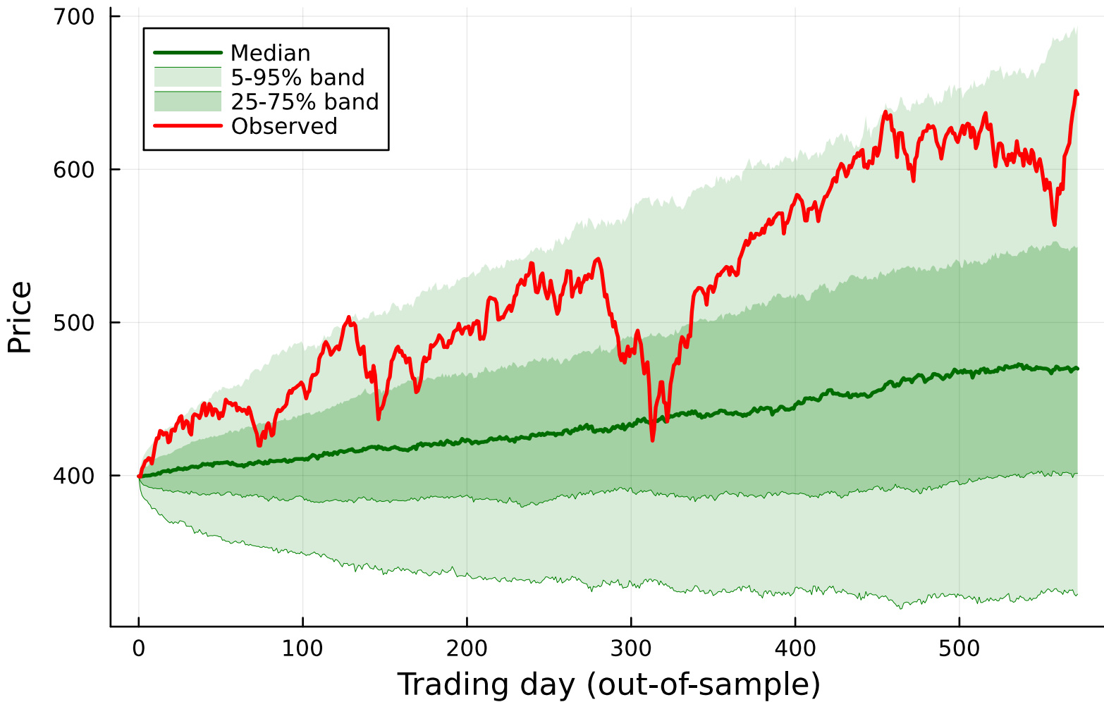
QQQ - VIX-cond. CHMM-N (K=18, 500 paths, lag=1)
