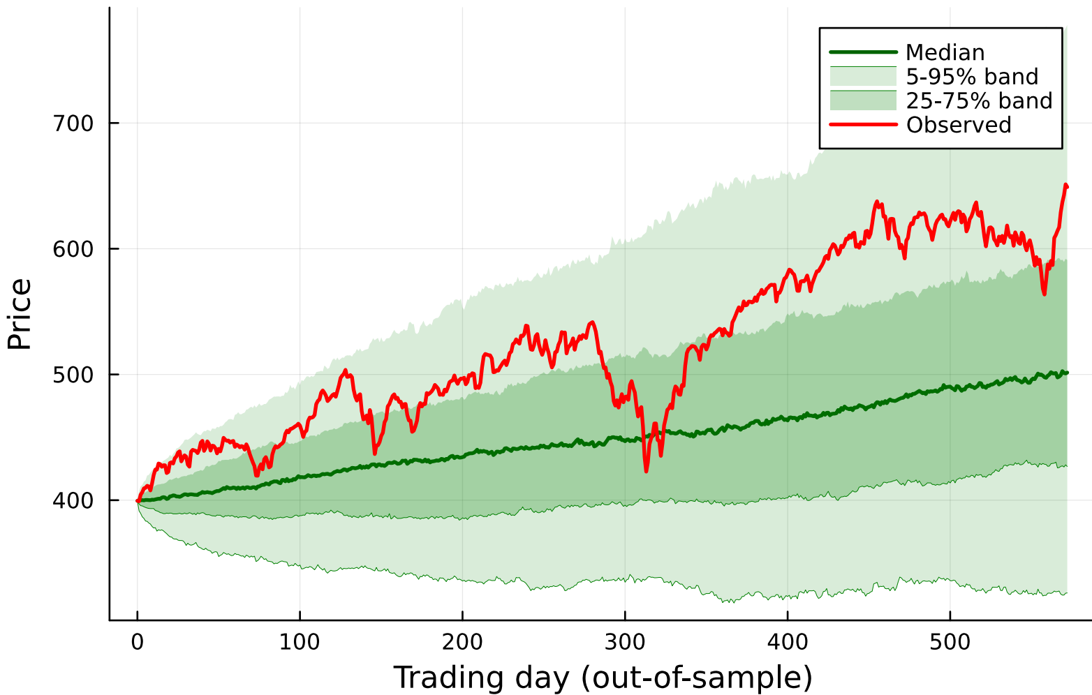
QQQ - VIX-cond. CHMM-t (K=18, 500 paths, lag=1)
