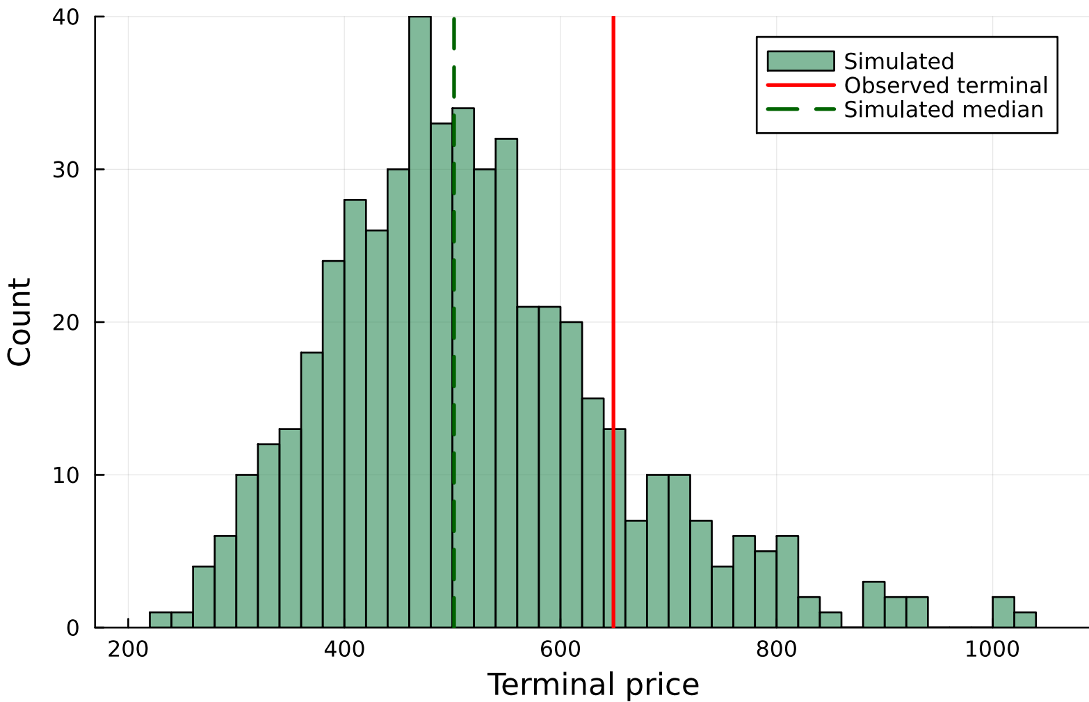
QQQ - VIX-cond. CHMM-t terminal (n=500)
