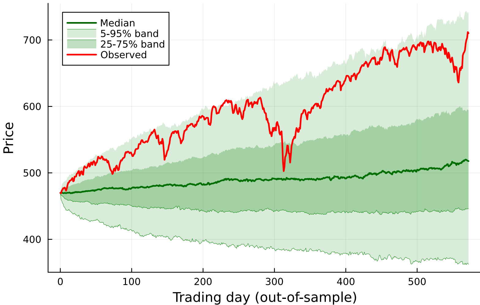
SPY - VIX-cond. CHMM-L (K=18, 500 paths, lag=1)
