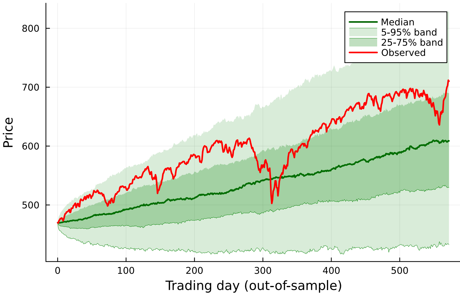
SPY - VIX-cond. CHMM-N (K=18, 500 paths, lag=1)
