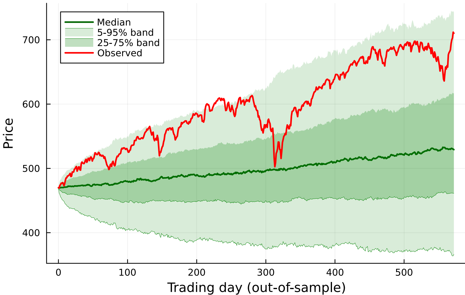
SPY - VIX-cond. CHMM-t (K=18, 500 paths, lag=1)
