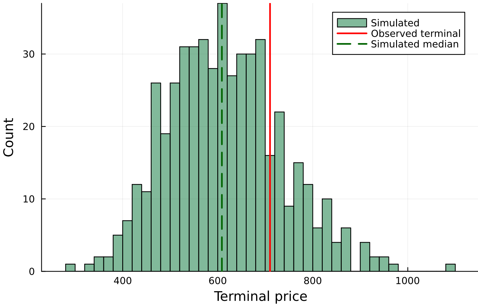
SPY - VIX-cond. CHMM-N terminal (n=500)
