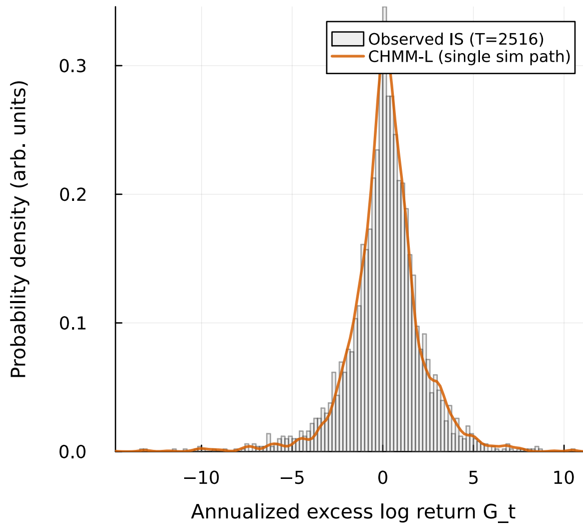
IS return density | KS pass rate = 94.2% of 1000 paths at alpha=0.05
