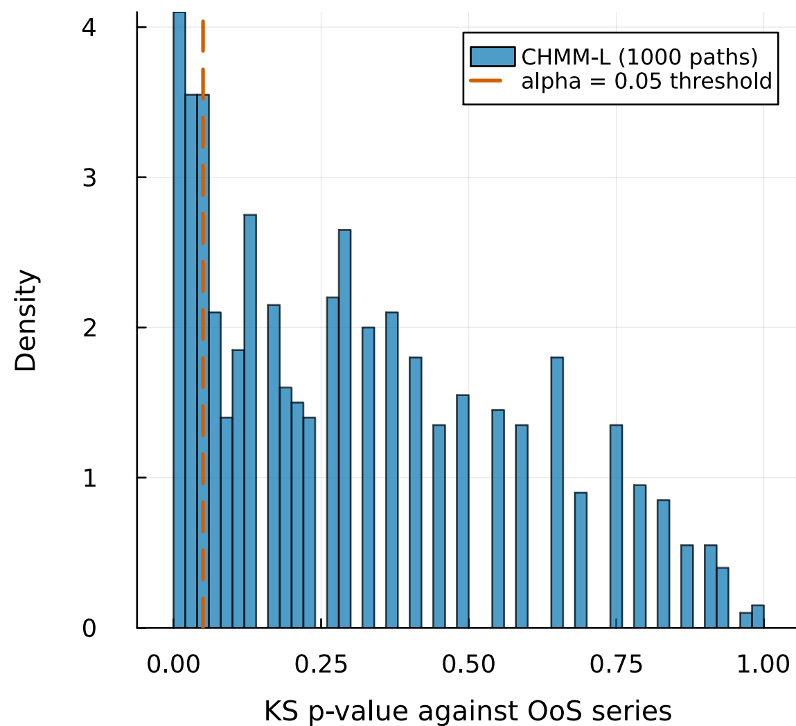
OoS KS p-values | pass rate = 80.5% above \alpha=0.05
