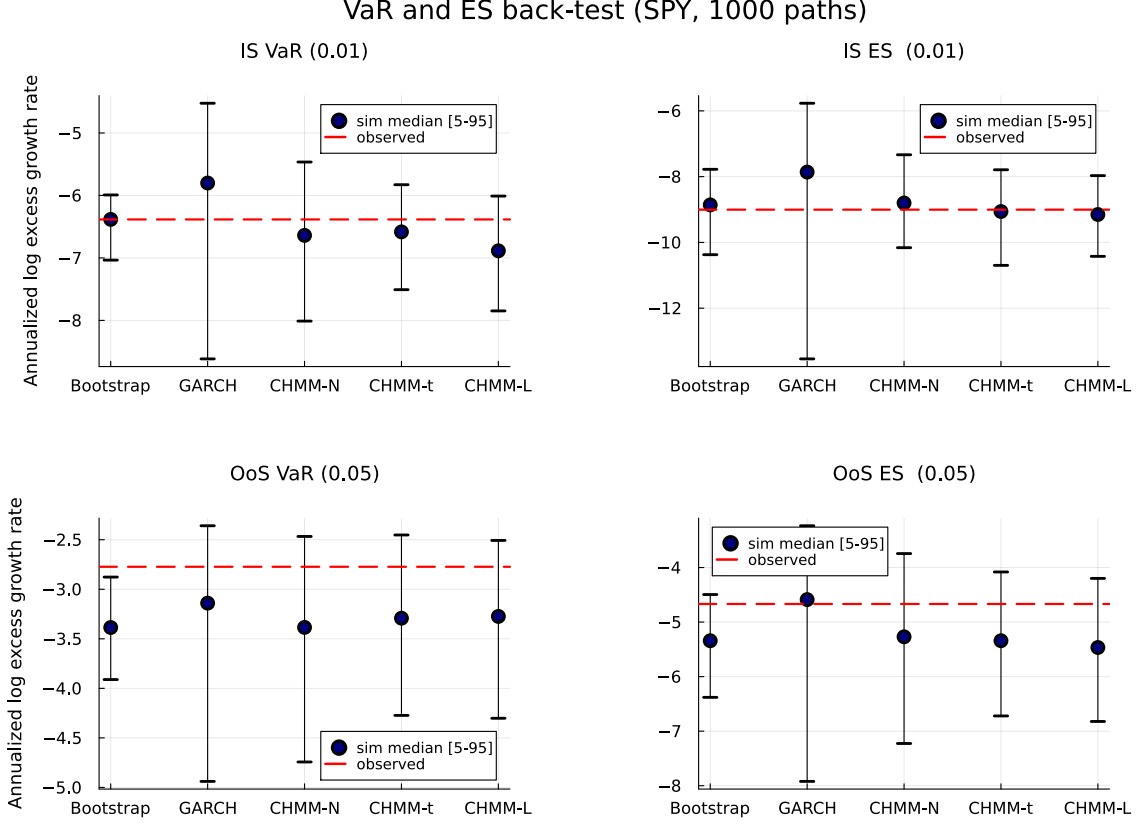
Figure 7. VaR / ES envelope diagnostic (SPY, N_{\text{paths}} = 1,000 ; global seed policy in Section 3.5). Each subplot shows the simulated median (dot) and [5%, 95%] envelope (error bar) across paths against the observed historical value (dashed red line); rows are IS and OoS windows, columns are VaR and ES, and the x-axis lists the five generators (Bootstrap, GARCH(1,1), CHMM-N, CHMM-t, CHMM-L). The y-axis is the annualized log excess growth rate (daily log return scaled by 1/\Delta t with \Delta t = 1/252 ), consistent with the R_{\text{IS}}/R_{\text{OoS}} convention used throughout the paper. Headline: every observed red line falls inside the corresponding simulated envelope, confirming that the CHMM family passes the coverage leg of the back-test complementary to the Kupiec likelihood-ratio leg in Section 4.6.
