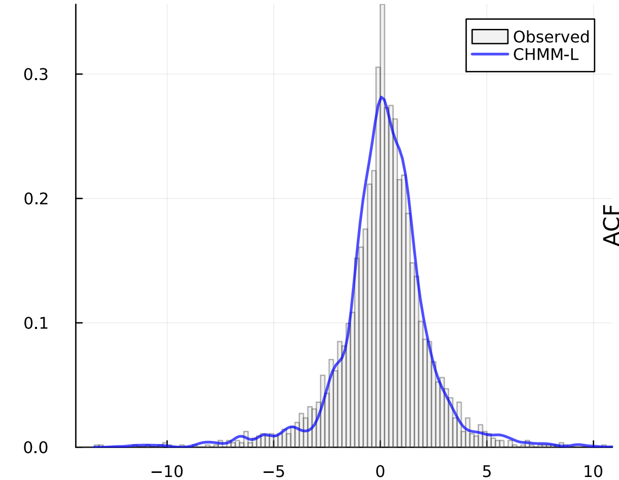
(a) IS Density (KS: 93.2%)
