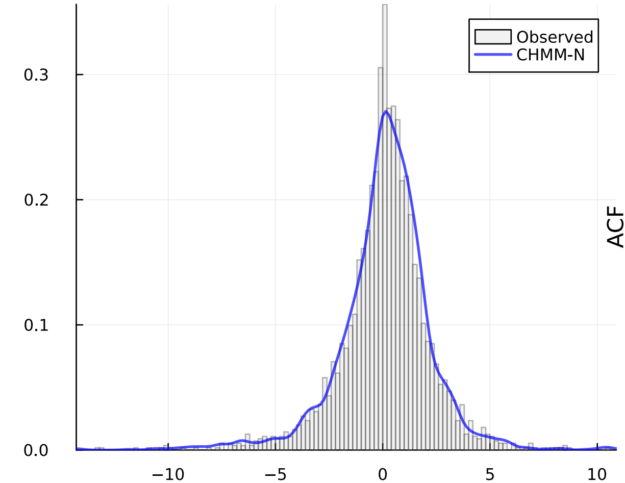
(a) IS Density (KS: 95.2%)
