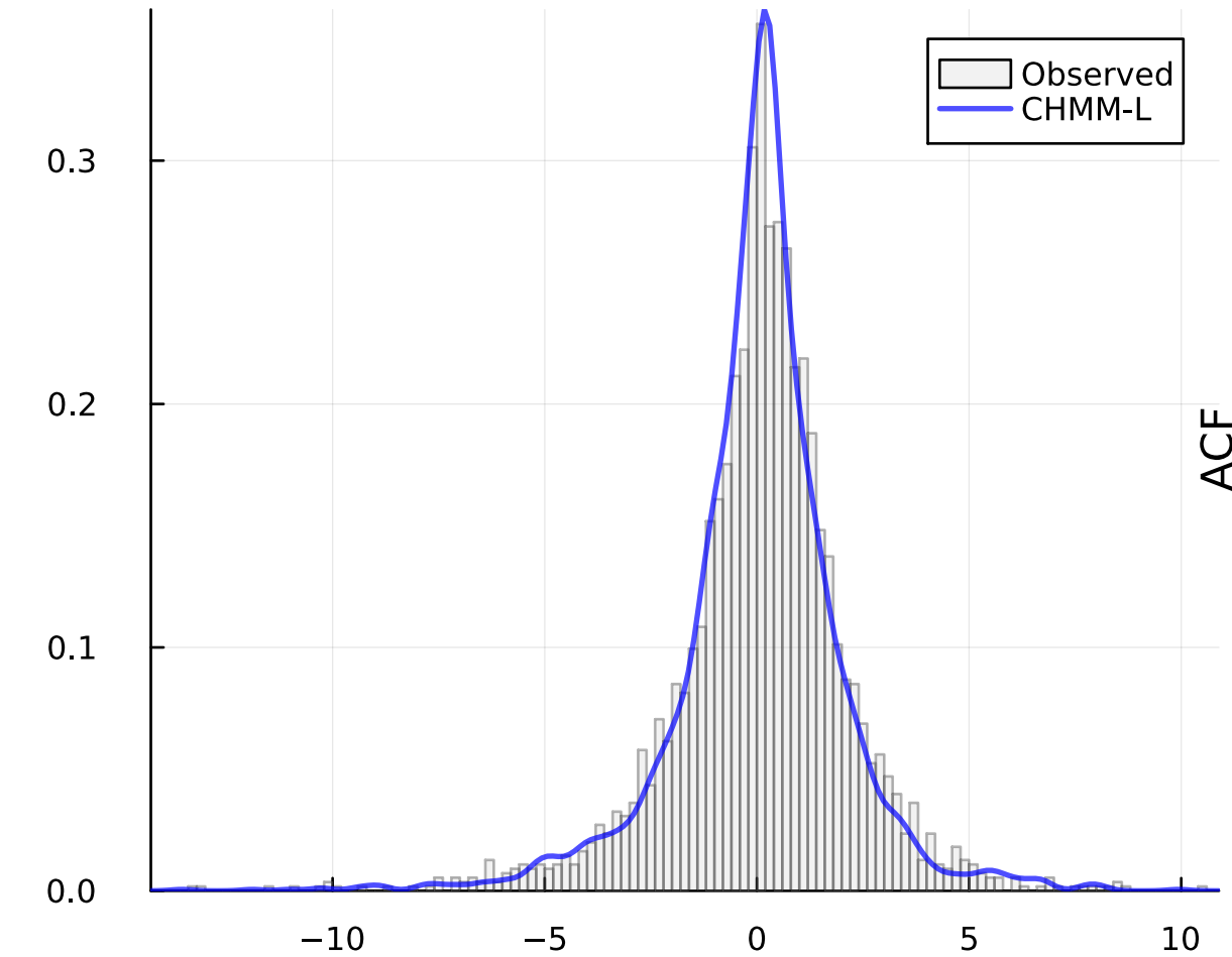
(a) IS Density (KS: 77.0%)
