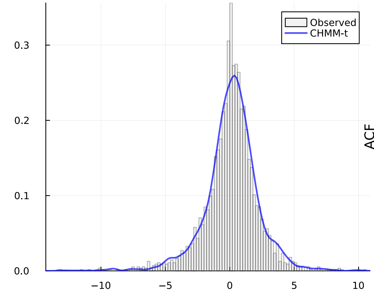
(a) IS Density (KS: 92.0%)
