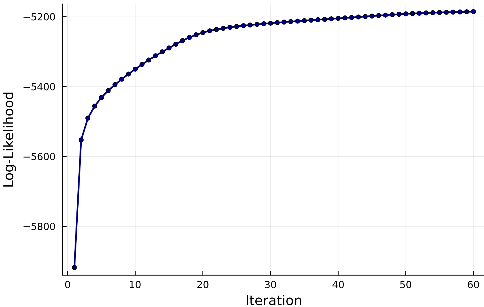
Convergence (CHMM-N, K=18)
