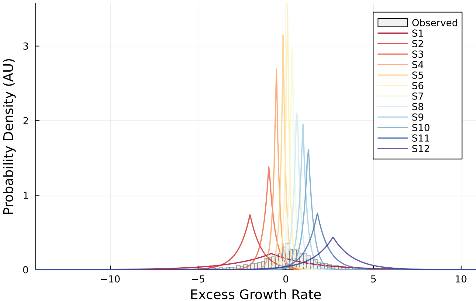
Emission Distributions (CHMM-L, K=12)
