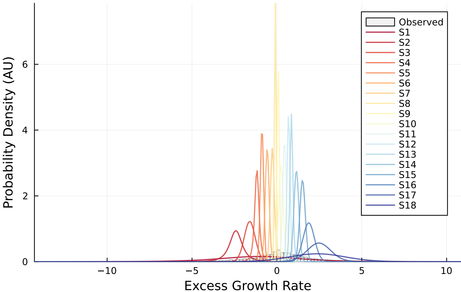
Emission Distributions (CHMM-t, K=18)
