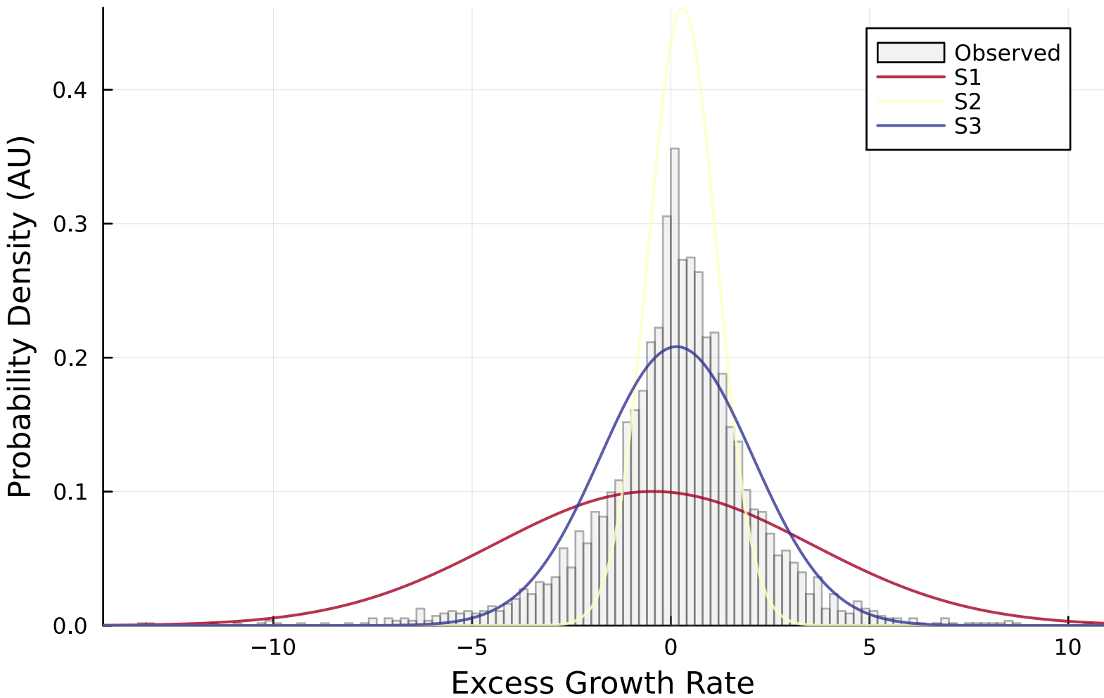
Emission Distributions (CHMM-N, K=3)
