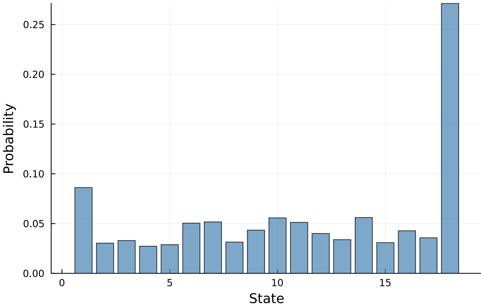
Stationary Distribution (CHMM-N, K=18)
