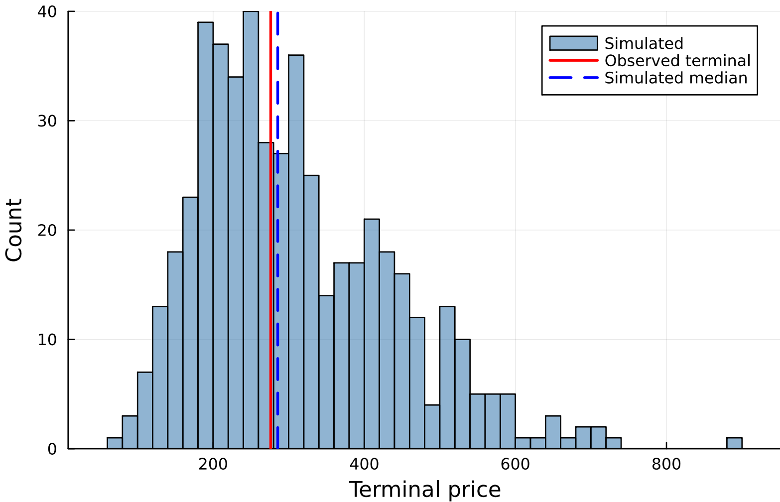
AAPL - CHMM-t terminal price (n=500)
