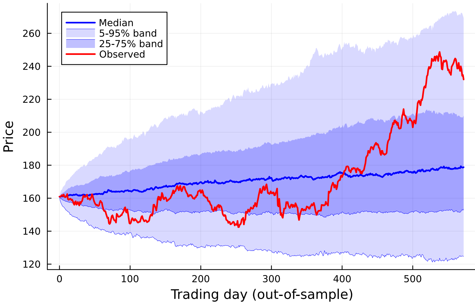
JNJ - CHMM-L price fan (K=18, 500 paths)
