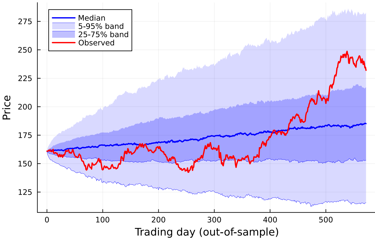
JNJ - CHMM-t pricefan (K=18, 500 paths)
