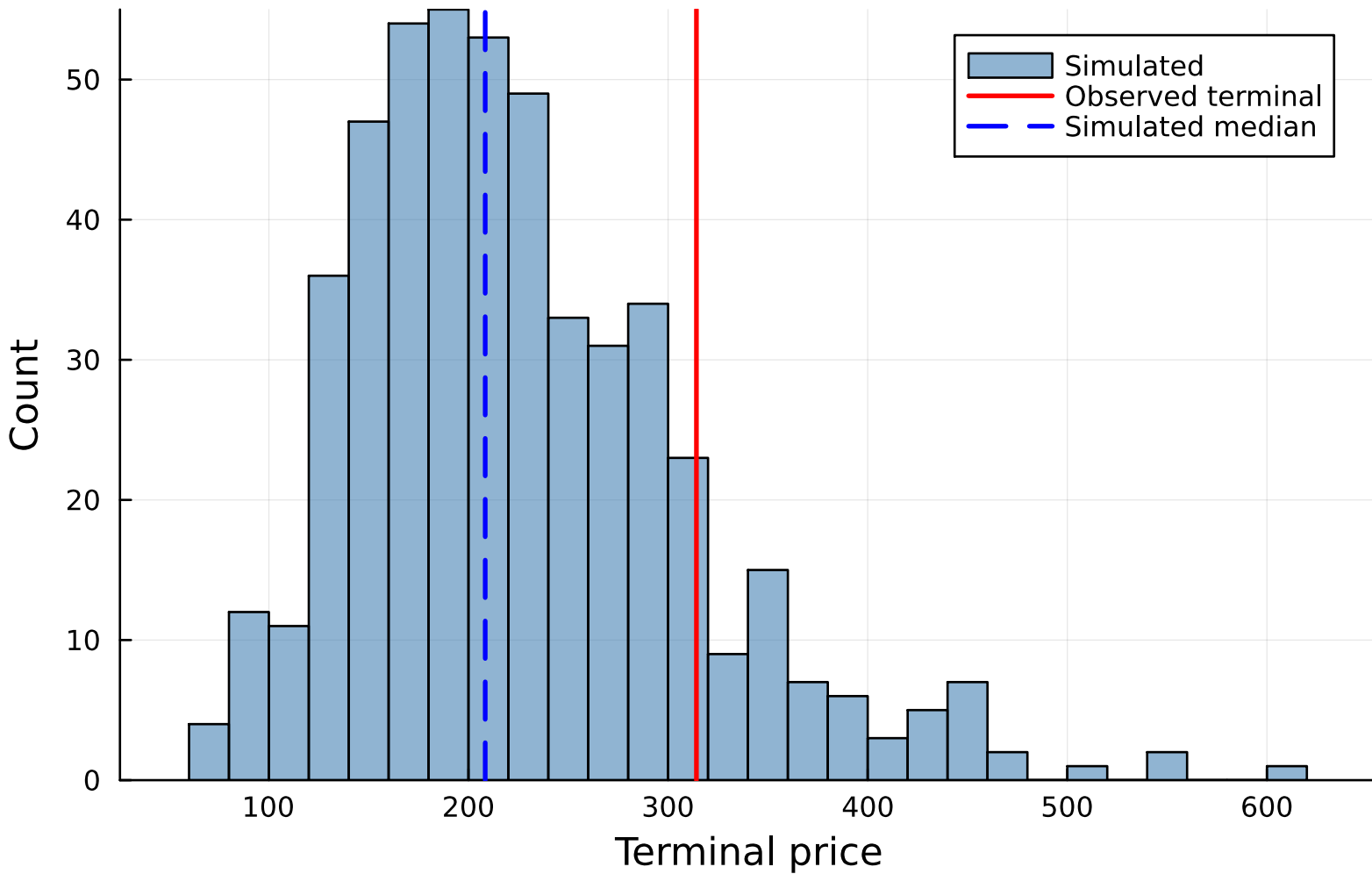
JPM - CHMM-L terminal price (n=500)
